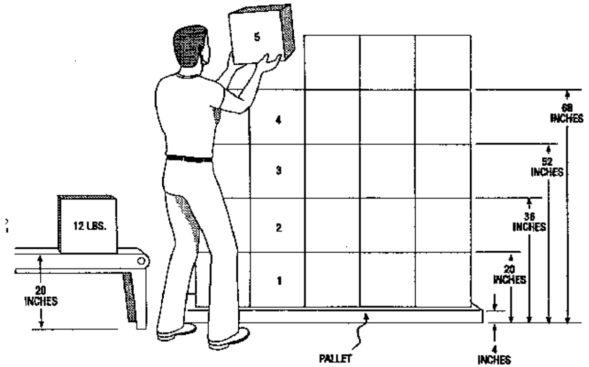
Figure 21 Depalletizing Operation, Example 7
