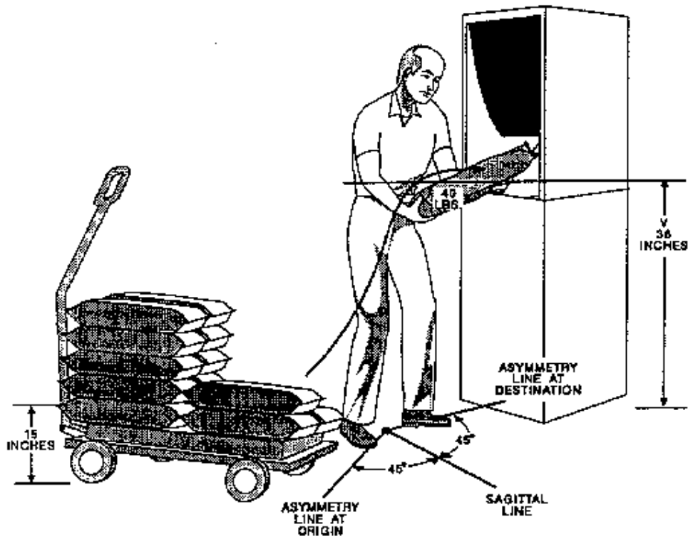
Figure 11 Loading Bags Into Hopper, Example 3
