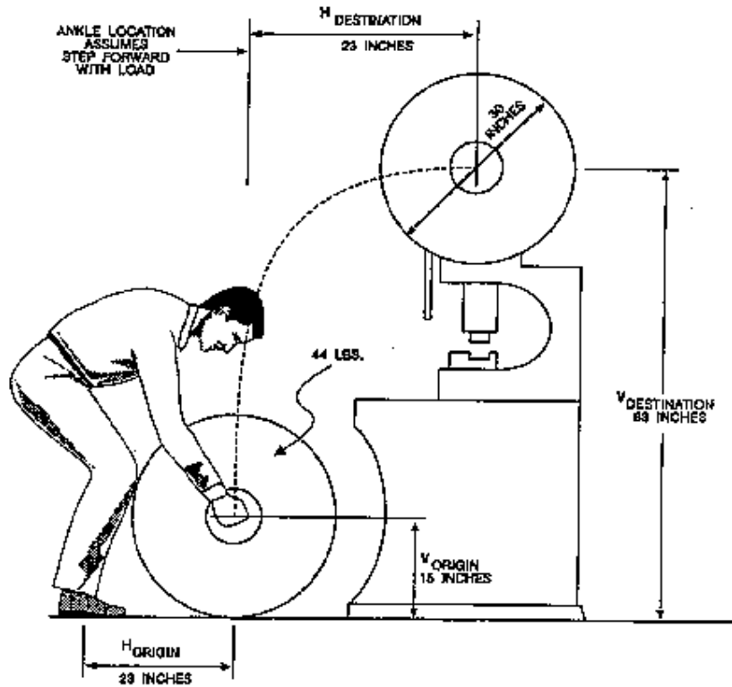
Figure 5 Loading Punch Press Stock, Example 1
