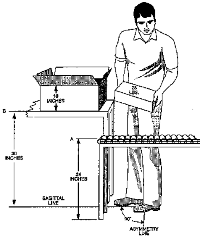
Figure 18 Packaging I, Example 6
