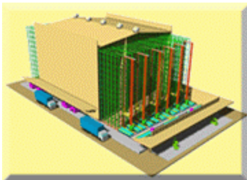
Samhwa Paint Industrial Co., Ltd.(Under construction) - 1 warehouse, Total 4,224 Cells, Stacker Crane 6 Sets
